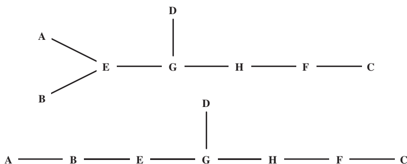
FIGURE 1. THE TWO PREFERENCE TREES THAT MAXIMIZE THE NUMBER OF VOTING PROFILES CONSISTENT WITH SINCERE VOTING AND SINGLE-PEAKED PREFERENCES
