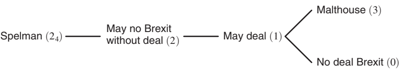
FIGURE 4. PREFERENCE TREE UNDERLYING THE FIRST VOTES ON BREXIT
