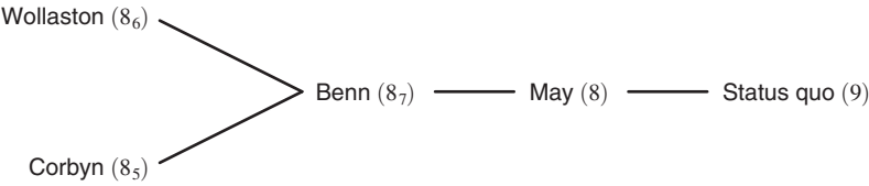
FIGURE 6. PREFERENCE TREE UNDERLYING THE SECOND BREXIT VOTE
