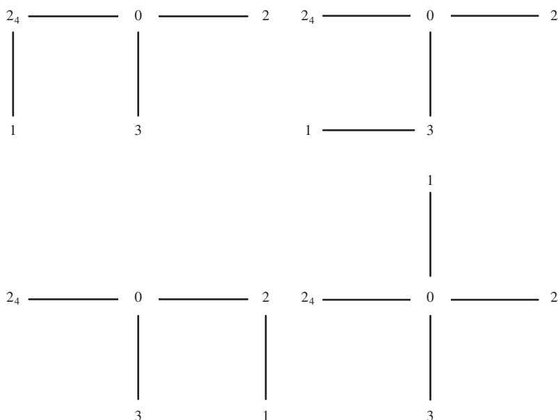
FIGURE 3. PREFERENCE TREES THAT YIELD A CONVEX AGENDA
